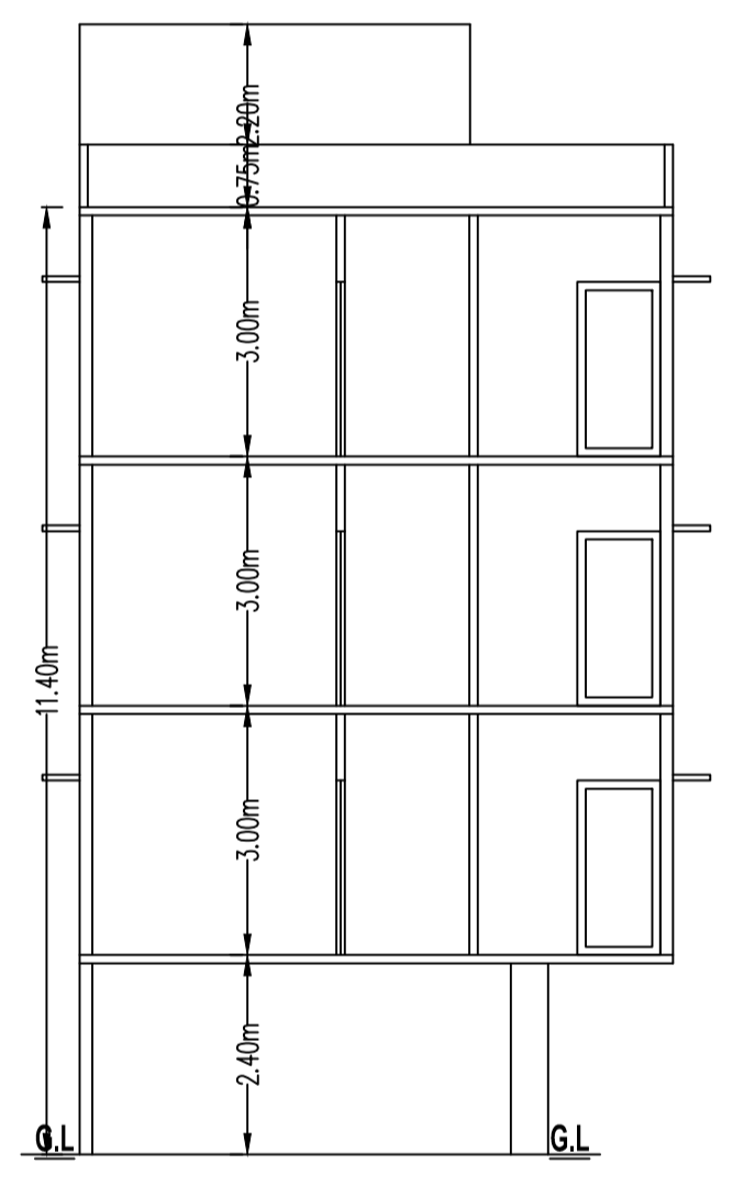
SECTION @ AA
